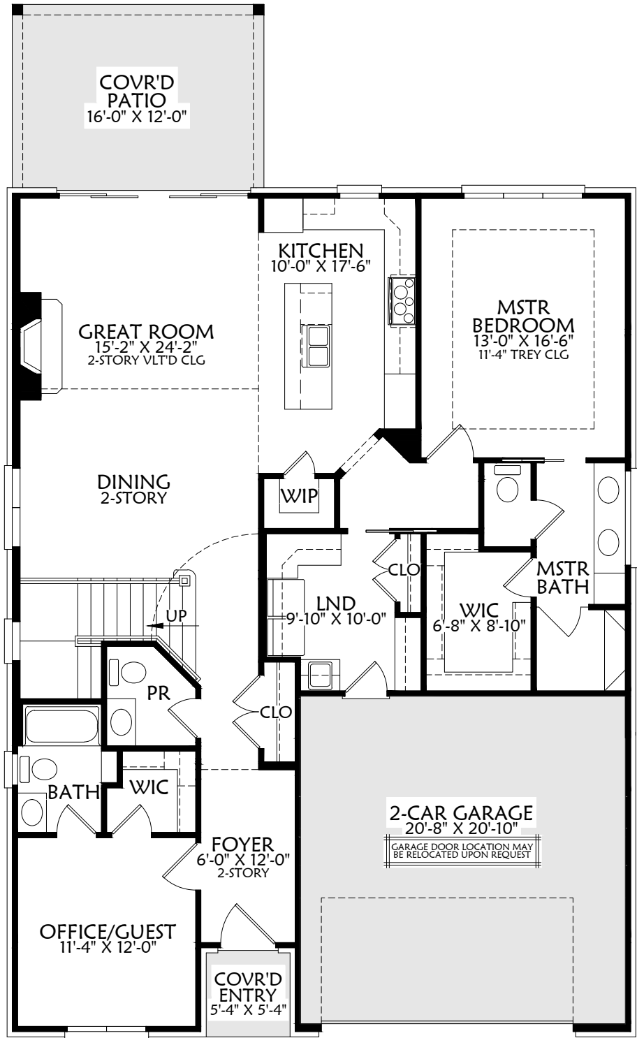
39'-4" MAIN FLOOR PLAN
